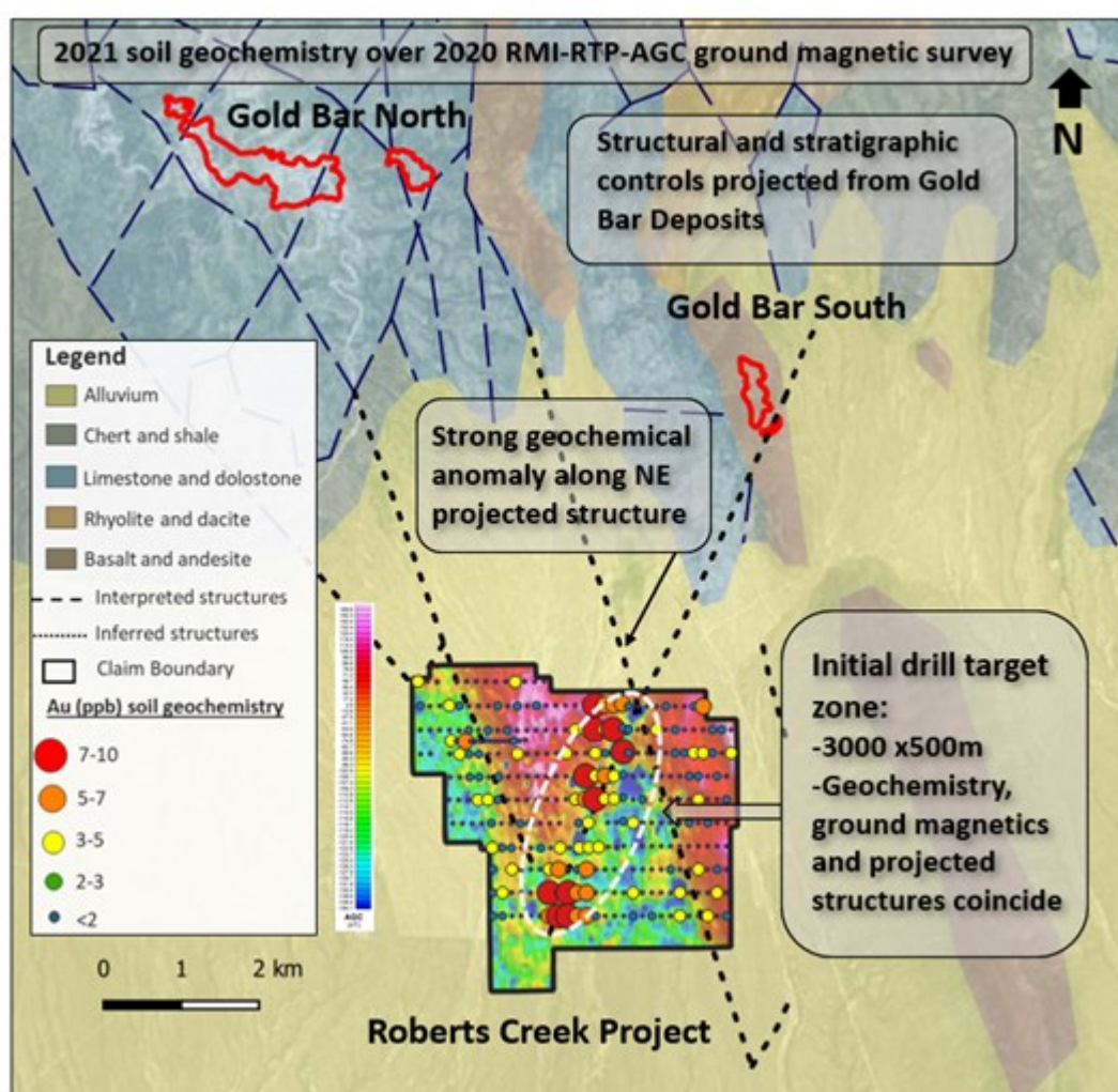
Figure 1: 2021 soil geochemistry superimposed over 2020 ground magnetic survey
