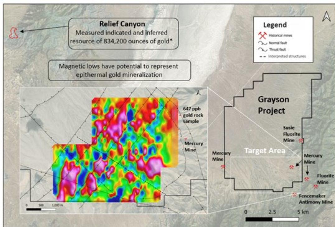
Figure 1. Orthophoto showing relative positions of the Grayson Project, the Relief Canyon Mine, and Mercury, Antimony, and Fluorite mines. Inset figure shows the well-defined correlation between major structures and the magnetic lows, which could be representative of alteration related to epithermal fluid flow and potential gold mineralization.
