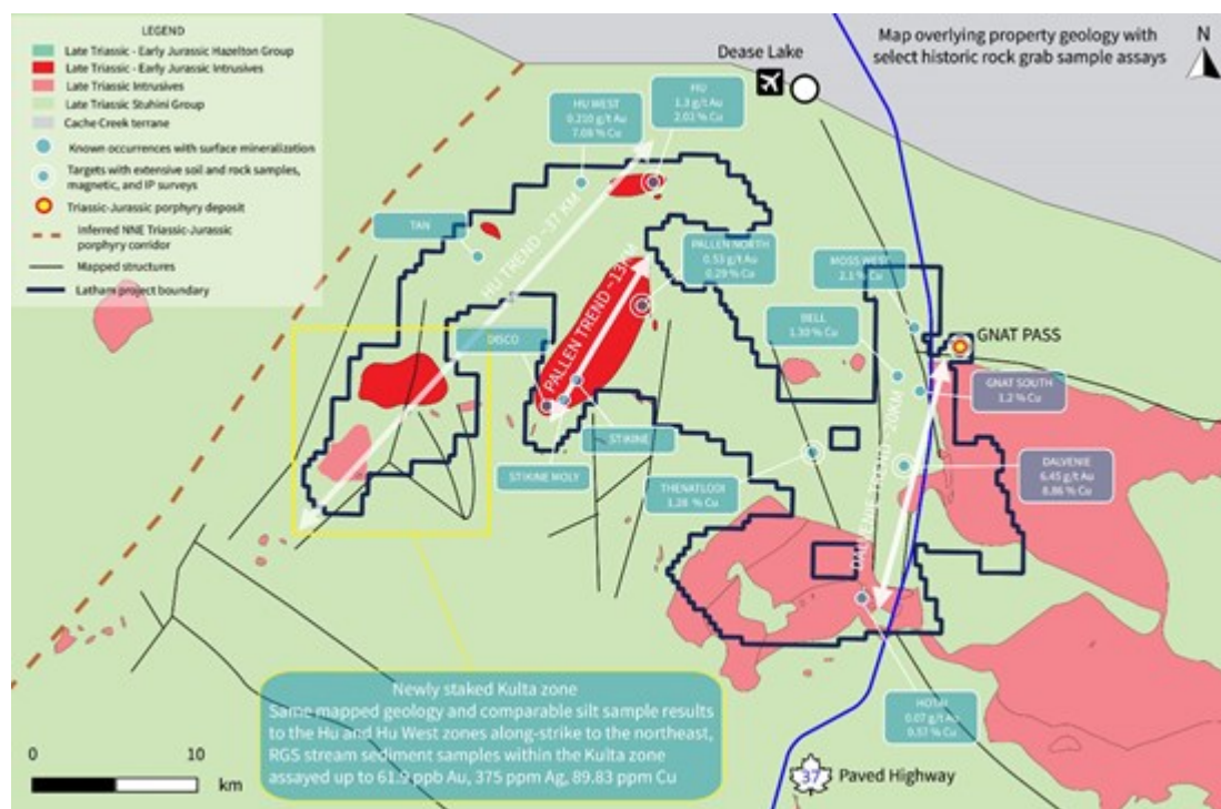
Figure 2. Latham trends to mineralization and known mineral occurrences.
