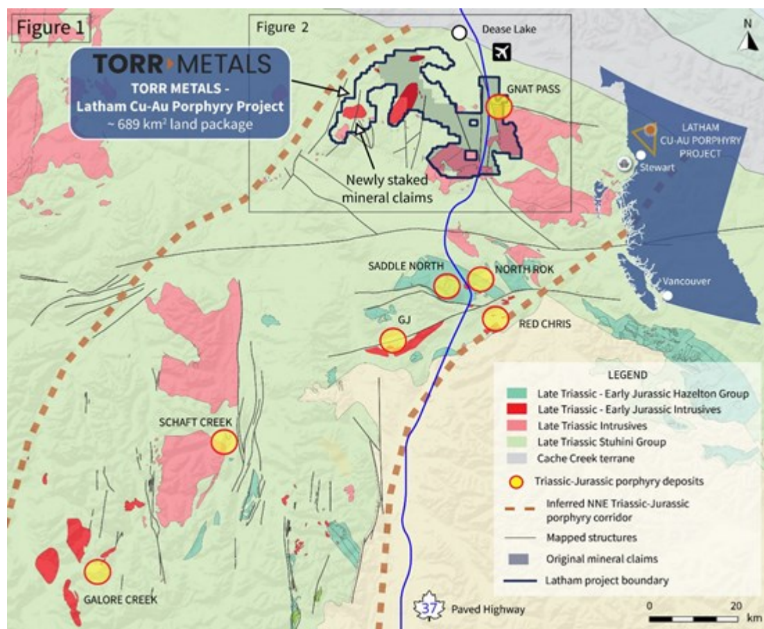
Figure 1. Latham Project and location of known Triassic and Jurassic porphyry deposits.
