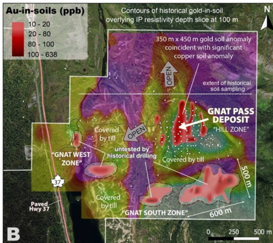
Figure 1.B. Gnat Pass Deposit area showcasing anomalous copper soil contours (A) and gold soil contours (B) based on historical soil sampling. Contours overlay IP resistivity depth slice at 100 m.
