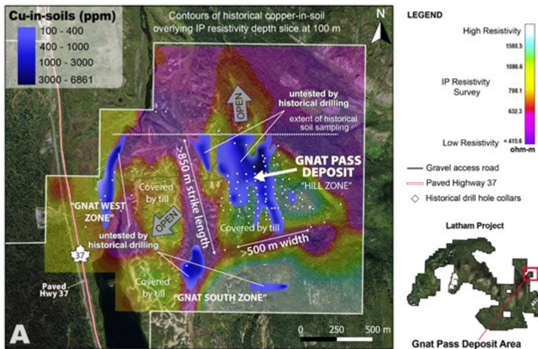
Figure 1.A. Gnat Pass Deposit area showcasing anomalous copper soil contours (A) and gold soil contours (B) based on historical soil sampling. Contours overlay IP resistivity depth slice at 100 m.
