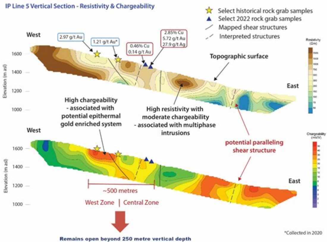
Figure 2B. 2022 IP survey line 5 with resistivity and chargeability in vertical section. Select assay values outlined in red (2022) and historical rock grab samples in blue (pre-2022).
