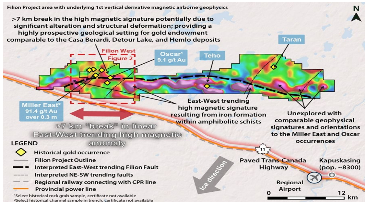
Figure 5. Filion Project location with underlying 1st derivative airborne magnetic geophysics at 200 m line spacing (Source: Canadian and Ontario Geological Surveys) annotated with historical gold occurrences, rock grab sampling, and structural interpretation.
