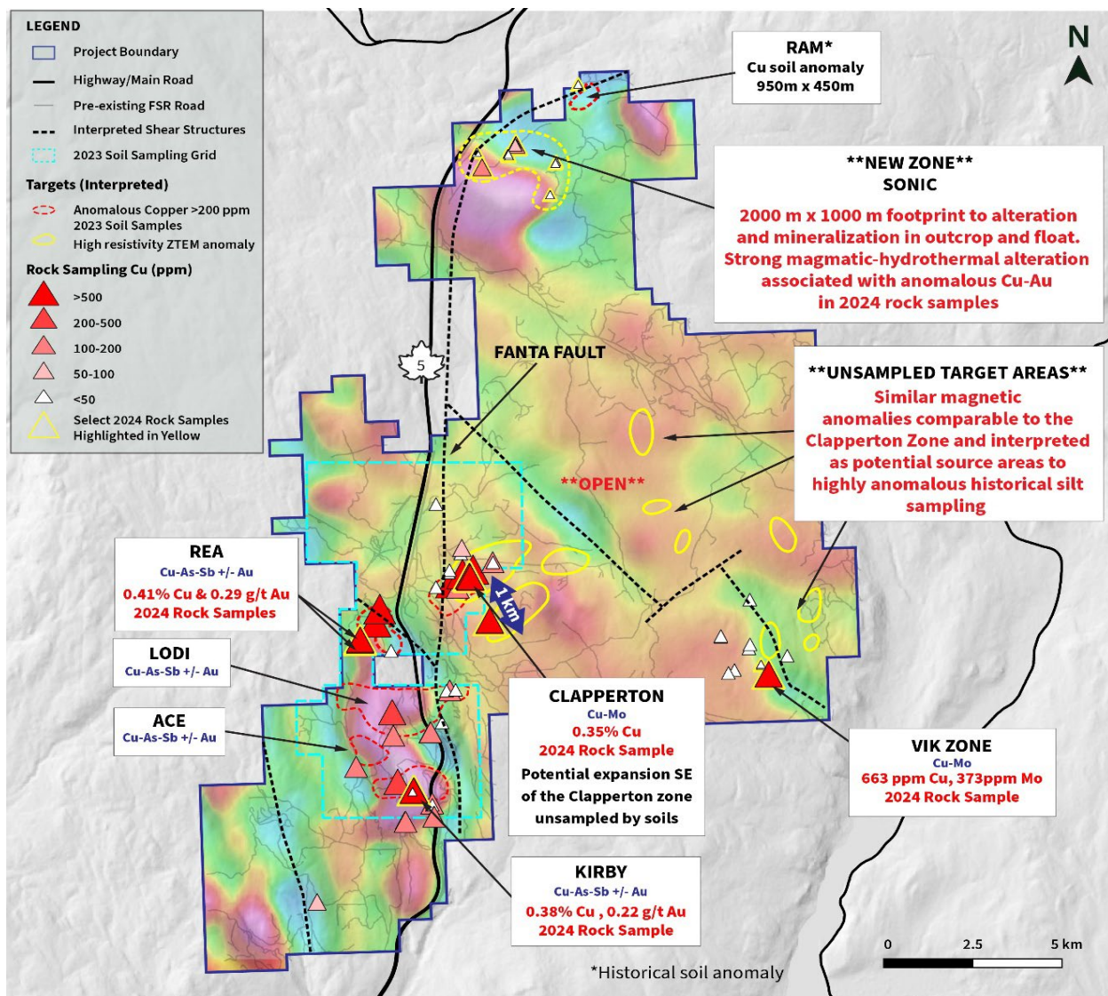
Figure 1. Soil and select rock grab sample results and target locations on the Kolos Project highlighting footprints to highly anomalous Cu in soil (>200 ppm), overlaying a regional RMI-VD geophysical survey.
