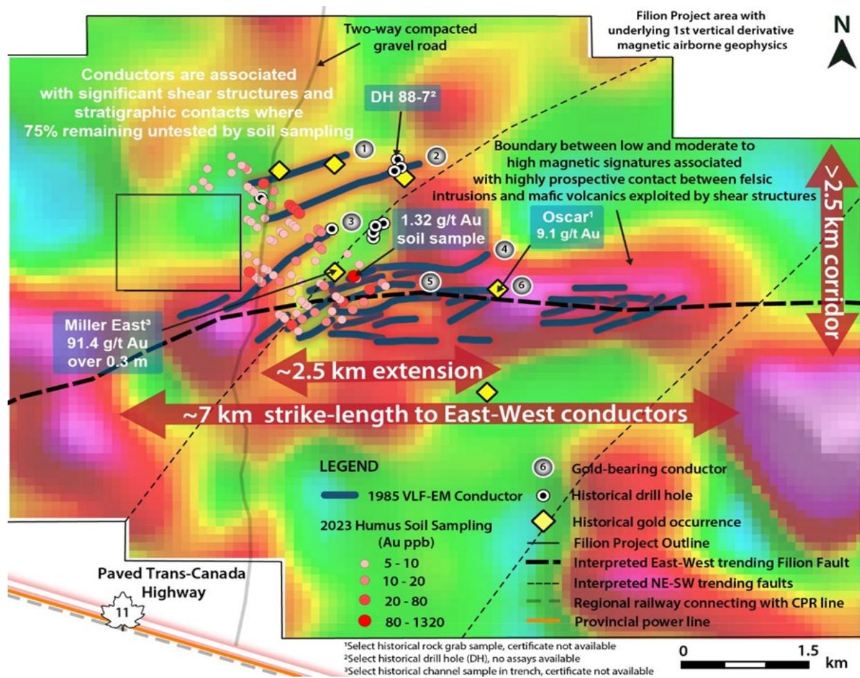
Figure 6. Filion West displaying location of anomalous gold in 2023 humus soil samples and 1985 VLF-EM conductors coincident with linear moderate to high magnetic signatures from airborne geophysics. Conductors occur within a highly prospective >7 km dilational bend of the Filion Fault, resulting in a “break” in the east-west trending high magnetic (iron formation) signature.
