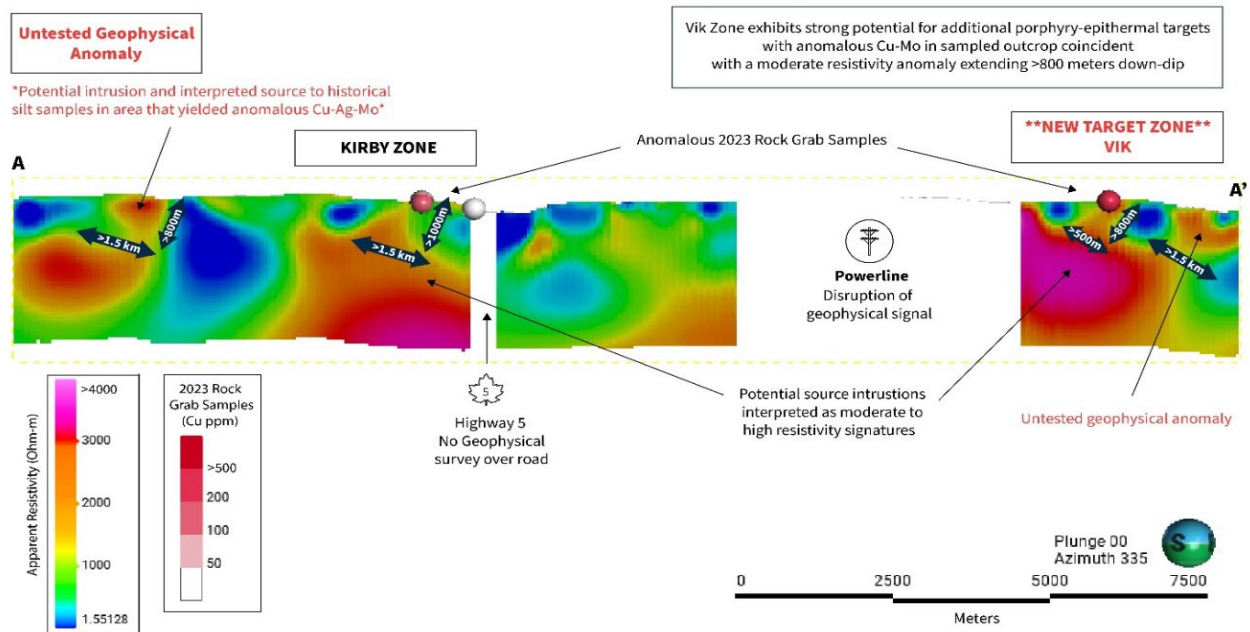
Figure 3. ZTEM 3D Resistivity Inversion Model voxel slice through the Kirby and Vik Zones. Additional untested geophysical exploration targets annotated to the southwest and northeast together with outlined dimensions of moderate to high resistivity targets that extend to-surface. View looking northwest.
