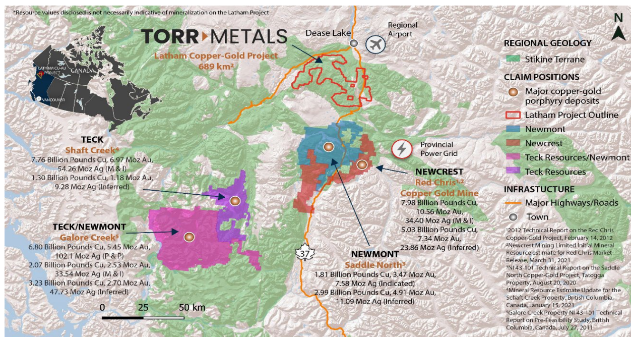
Figure 7. Regional geology showcasing the Stikine Terrane, Latham project location, and nearby major copper-gold porphyry deposits.
