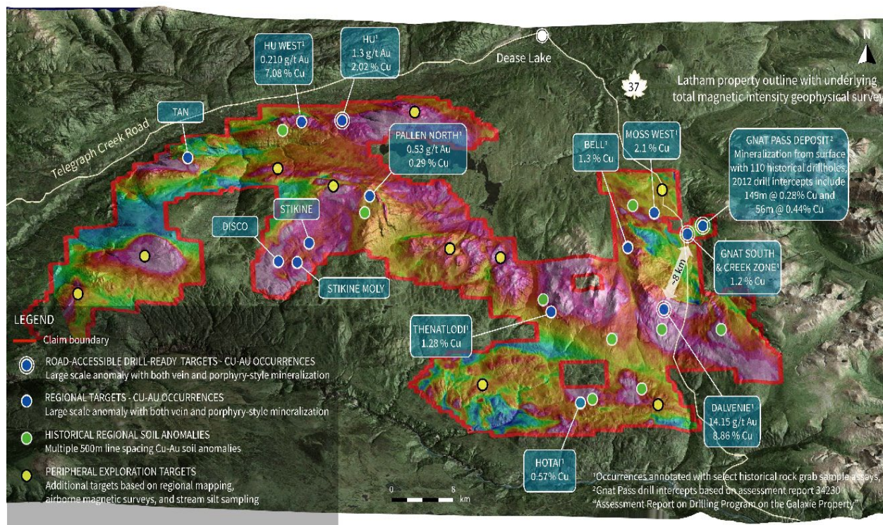
Figure 8. Latham Project location with airborne total magnetic survey data and mineral occurrences.
