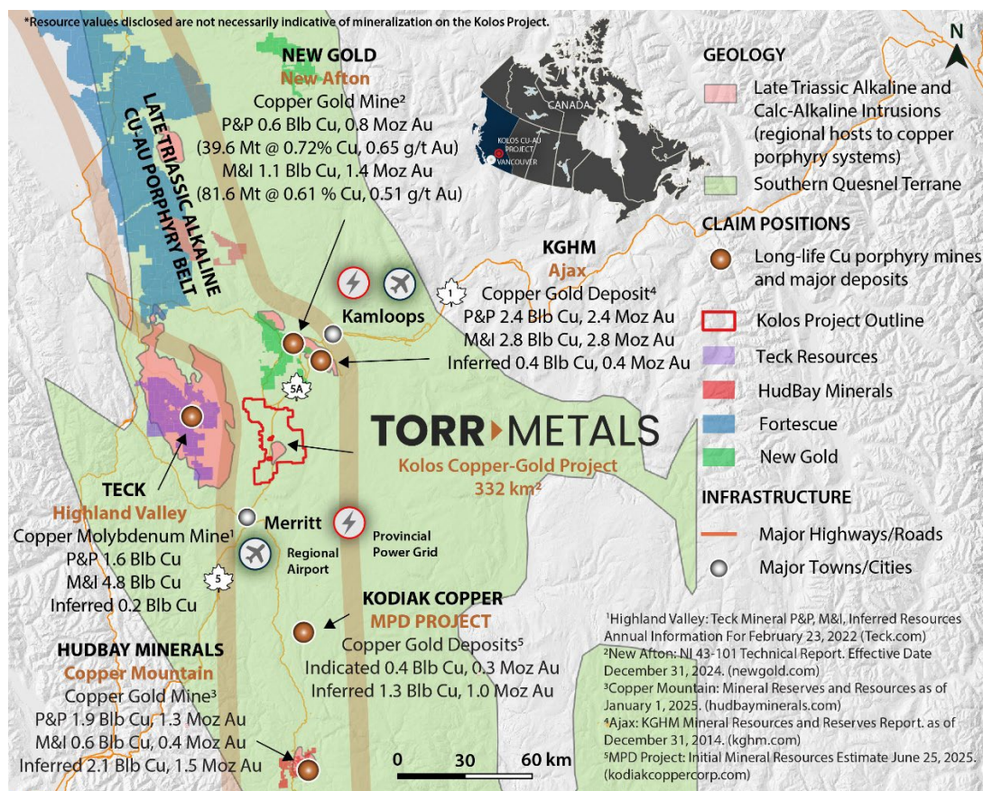
Figure 1. Kolos Copper-Gold Project location within the prolific Late Triassic porphyry belt of the Quesnel Terrane in south-central British Columbia. Figure modified from Mitchinson et al. 2024.
