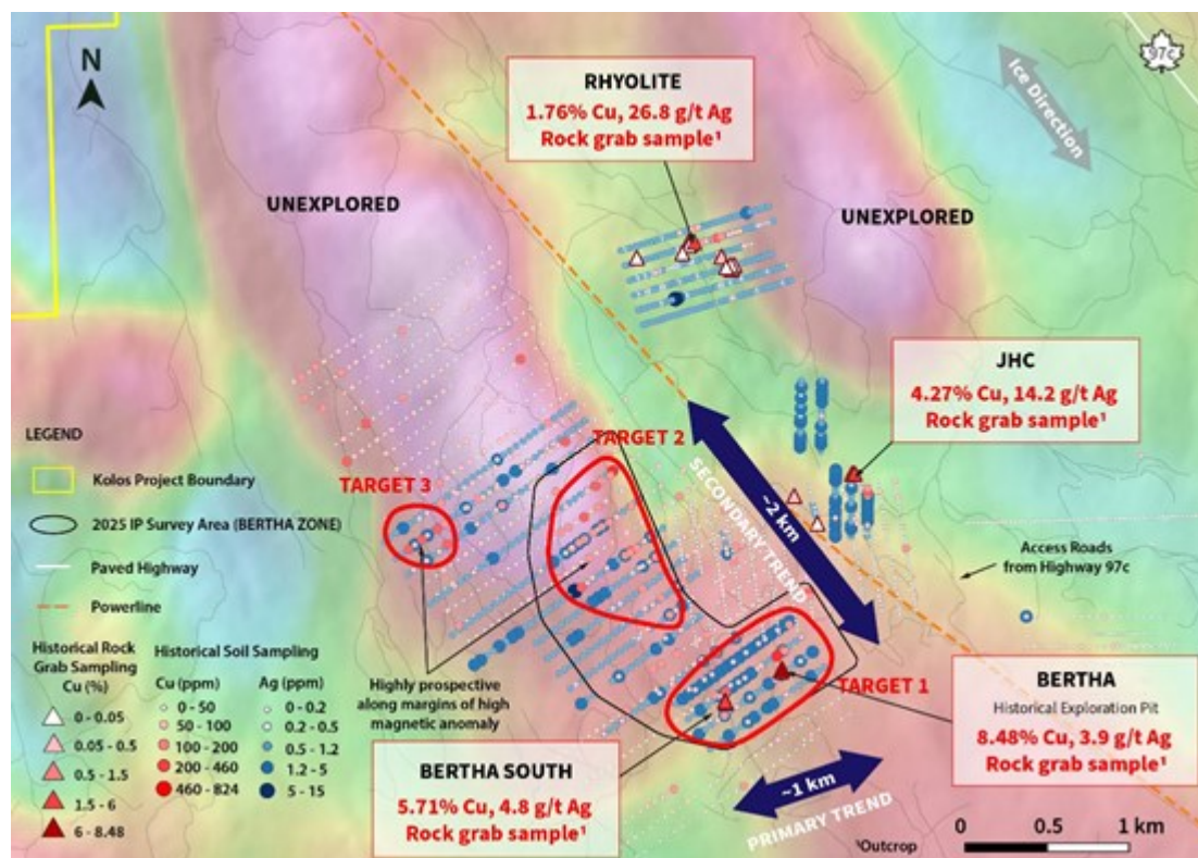
Figure 2. Historical soil and rock grab samples outlining anomalous Cu and Ag overlying the vertical derivative of residual magnetic intensity (RMI) geophysics with select annotated rock grab samples.
