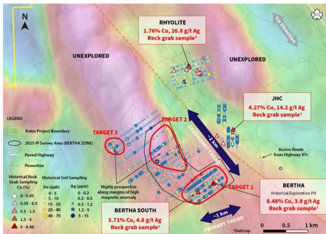
Figure 3. Historical soil and rock grab samples outlining anomalous Cu and Au overlying the vertical derivative of residual magnetic intensity (RMI) geophysics with select annotated rock grab samples.
