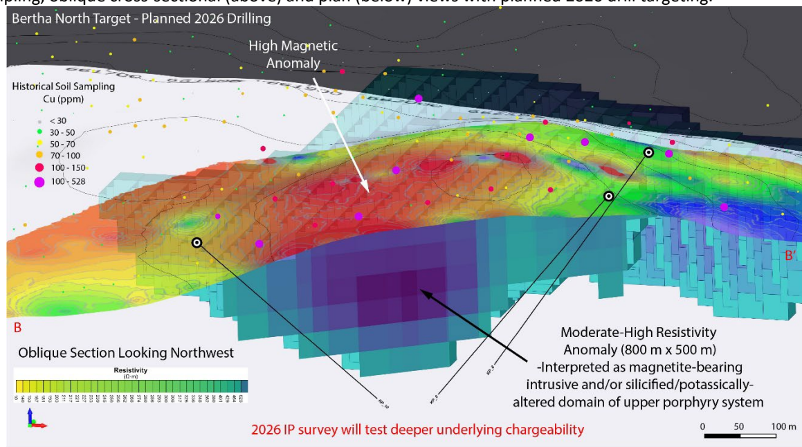
Figure 2. 2025 inverted IP resistivity and overlying magnetic geophysical survey with historical copper-gold soil sampling, oblique cross-sectional (above) and plan (below) views with planned 2026 drill targeting.
