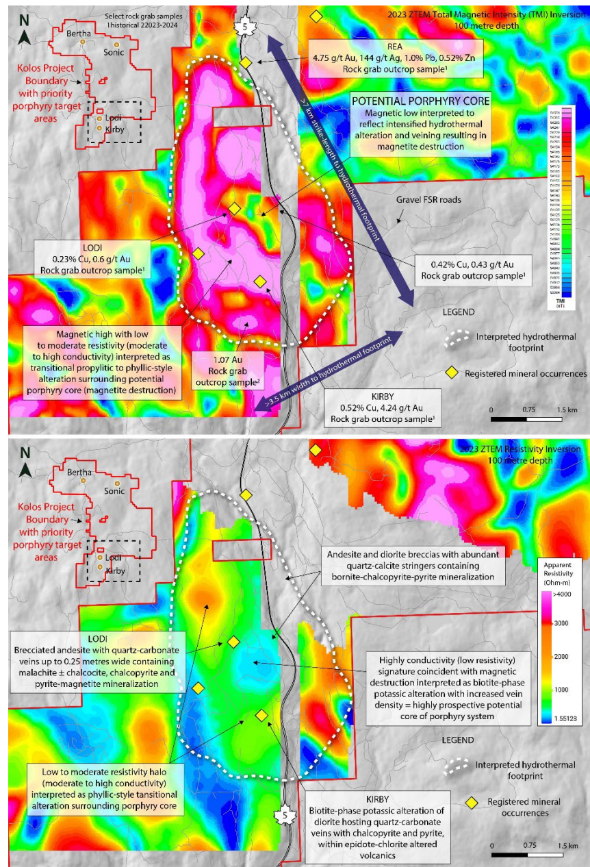
Figure 1. Newly inverted 2023 ZTEM total magnetic intensity (TMI) (above) and resistivity (below) geophysical surveys with outlined hydrothermal footprint, annotated registered mineral occurrences, and select rock grab samples.
