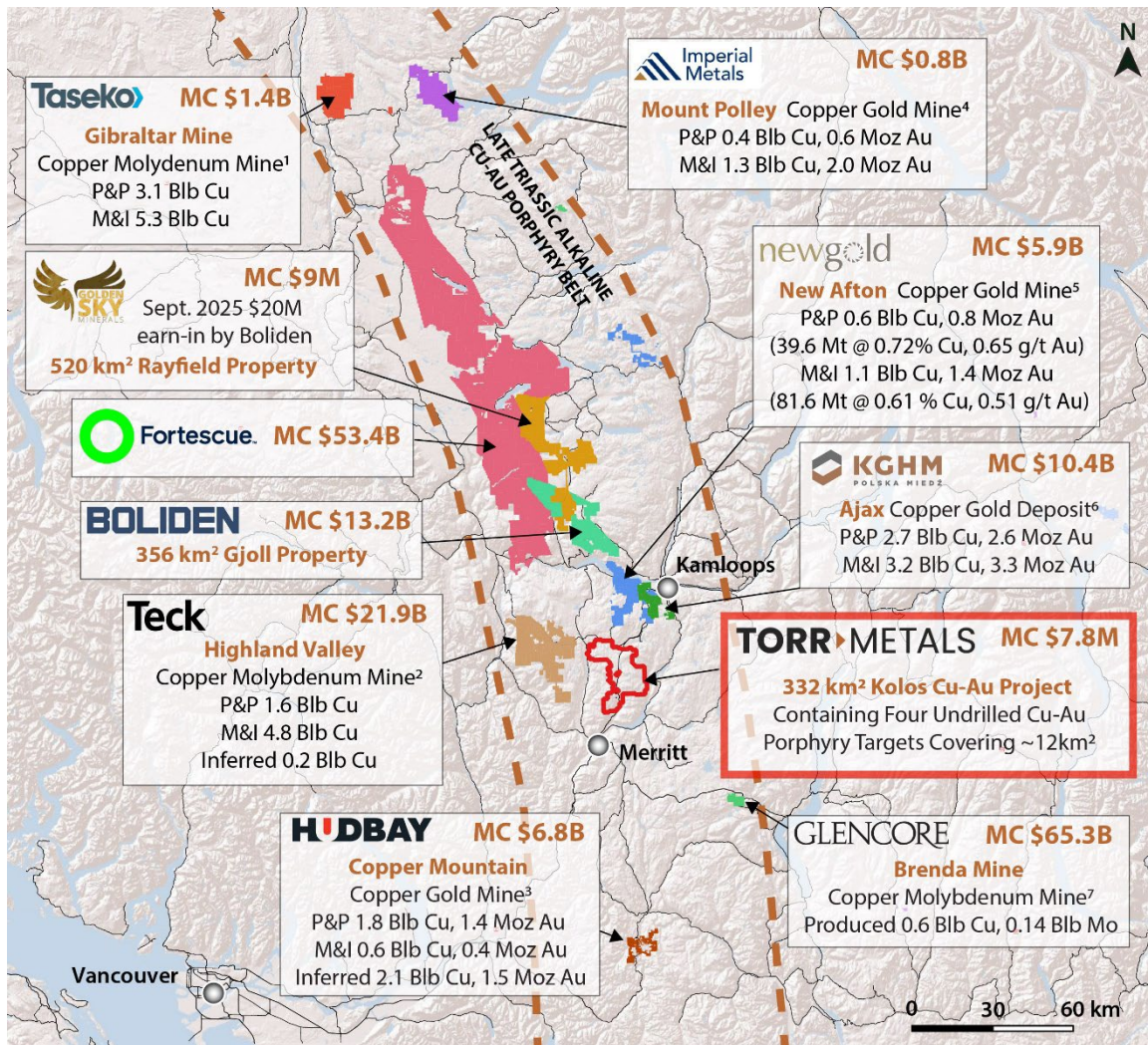
Figure 4. Project location within the southern Quesnel Trough porphyry trend, figure showcases the nearby land positions and assets held by major mining companies and recent transactions.
